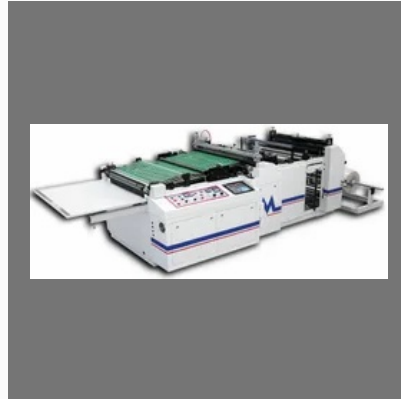
High Speed Side Seal Bag Maker WIN 750P
